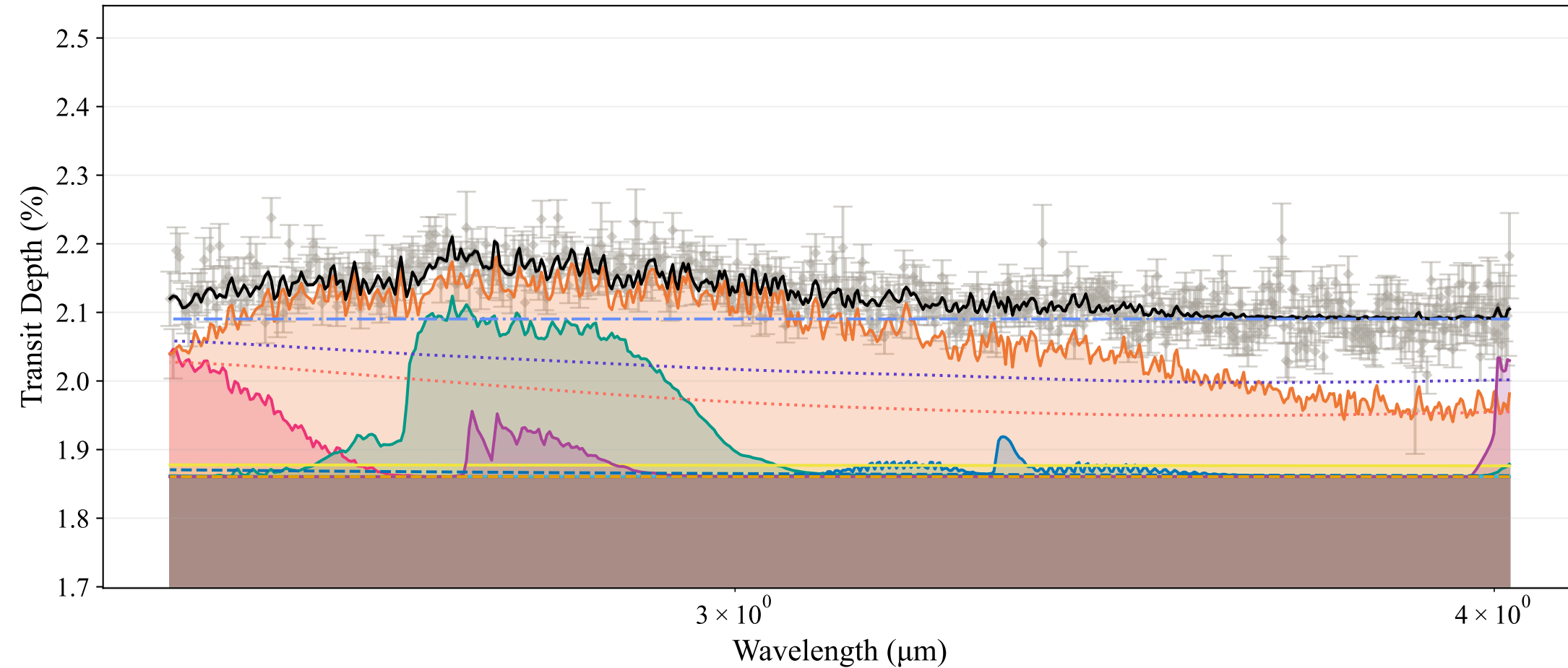
NIRCAM, SiO, Isothermal
